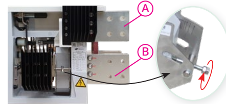
Setting of maximum current release
