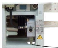
Setting of maximum current release
